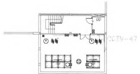
SECURITY SYSTEM LAYOUT - BASEMENT FLOOR PLAN SCALE: 1:200
