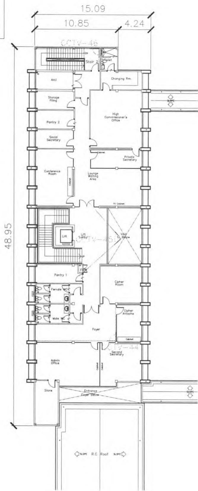
SECURITY SYSTEM LAYOUT - FIRST FLOOR PLAN SCALE: 1:200
